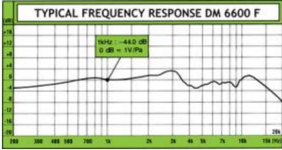
TYPICAL FREQUENCY RESPONSE DM 6600 F
